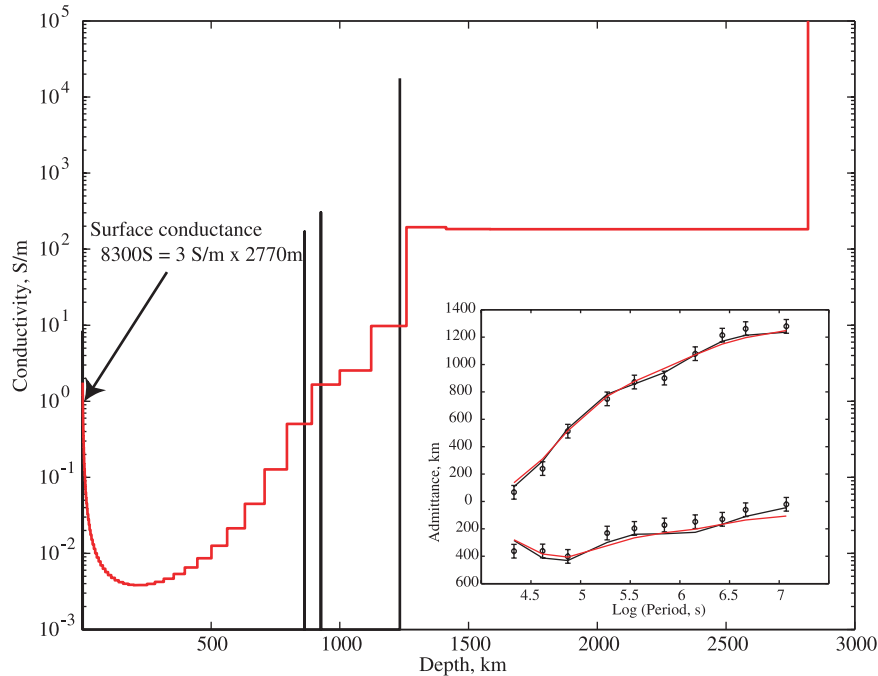
Figure 10. Models generated by Occam smooth inversion (stepped red line) fitting to RMS 1.15 and a graphical representation of the D^+ model (vertical bars), which fits the data to RMS 0.95, and plotted assuming a layer thickness of 1/1000 of a decade (i.e., 1 km at a depth of 1000 km) and a conductivity scaled by 1/1000. The D^+ model includes a delta function at the surface of conductance 8300 S. The inset shows fits to the data set for both these models.
