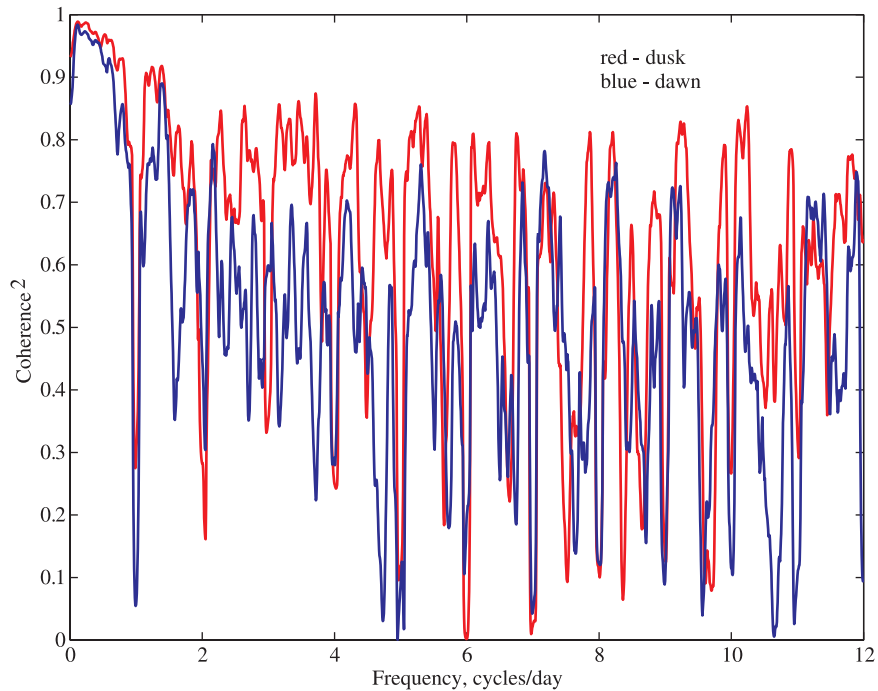
Figure 7. Coherence spectra between e_1^0(t) and i_1^0(t) for the dawn and dusk timeseries. Coherences are higher for the dusk data, but drop at harmonics of one day, presumably because of contamination from ionospheric sources.
