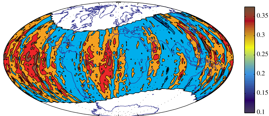
Figure 11. Global induction obtained by combining B_r and B_\theta components of normalized induced field, averaged in 2 \times 3^\circ bins.
