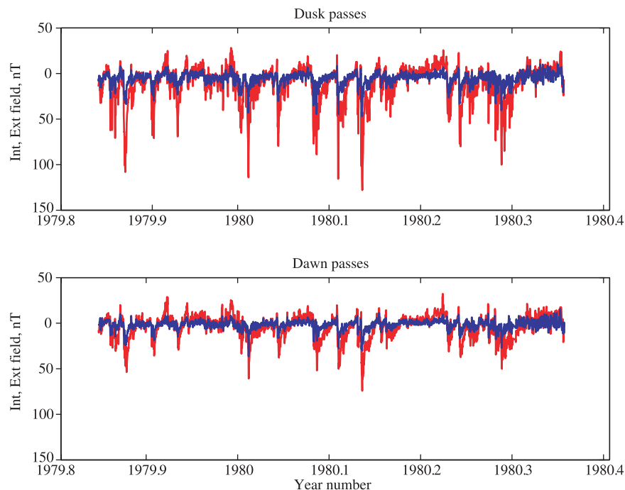
Figure 3. Least squares estimates of i_1^0(t) (blue) and e_1^0(t) (red) from CMP3-Dst residuals. The upper plot is for dusk passes, lower for dawn.
