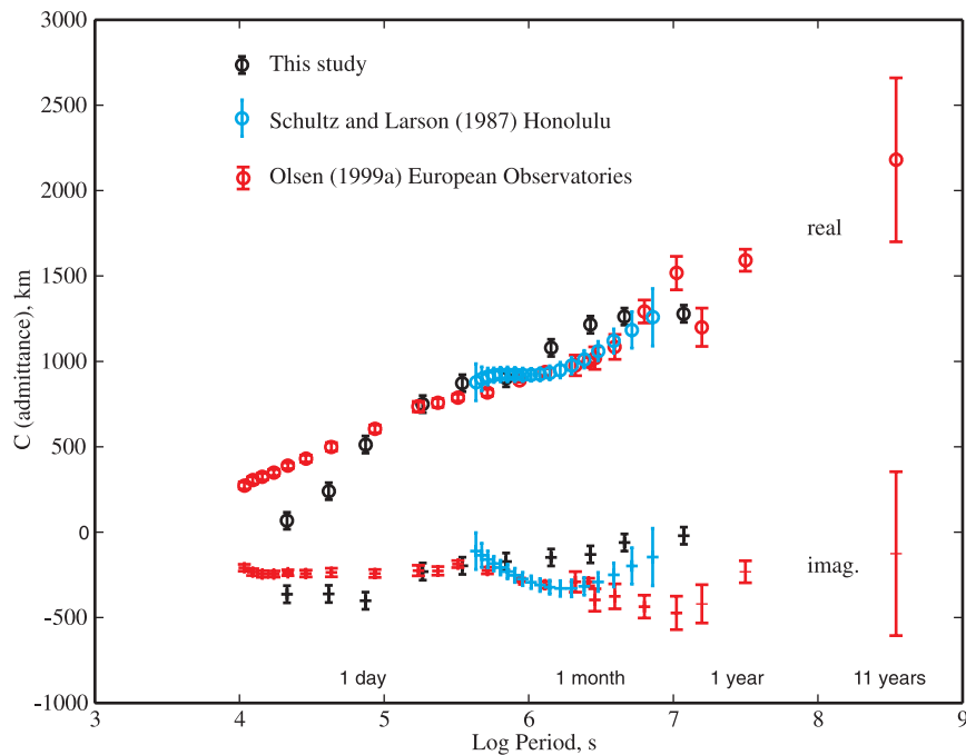
Figure 9. Our Magsat 1-D response function (black), the European observatory average of Olsen [1999a] (red) which includes the 11 year estimate of Harwood and Malin [1977], and Schultz and Larsen's [1987] response for the Honolulu observatory (blue).
