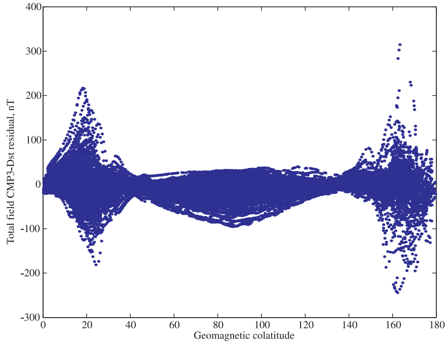
Figure 1. A sample of CMP3-Dst residuals (the first 100,000 data points) for the total magnetic field plotted as function of geomagnetic colatitude, \theta_d . We use only observations in colatitude range 40^\circ < \theta_d < 140^\circ for our modeling to avoid magnetic fields associated with field-aligned currents, here evident as rapidly varying fields peaking within 20^\circ of the poles.
