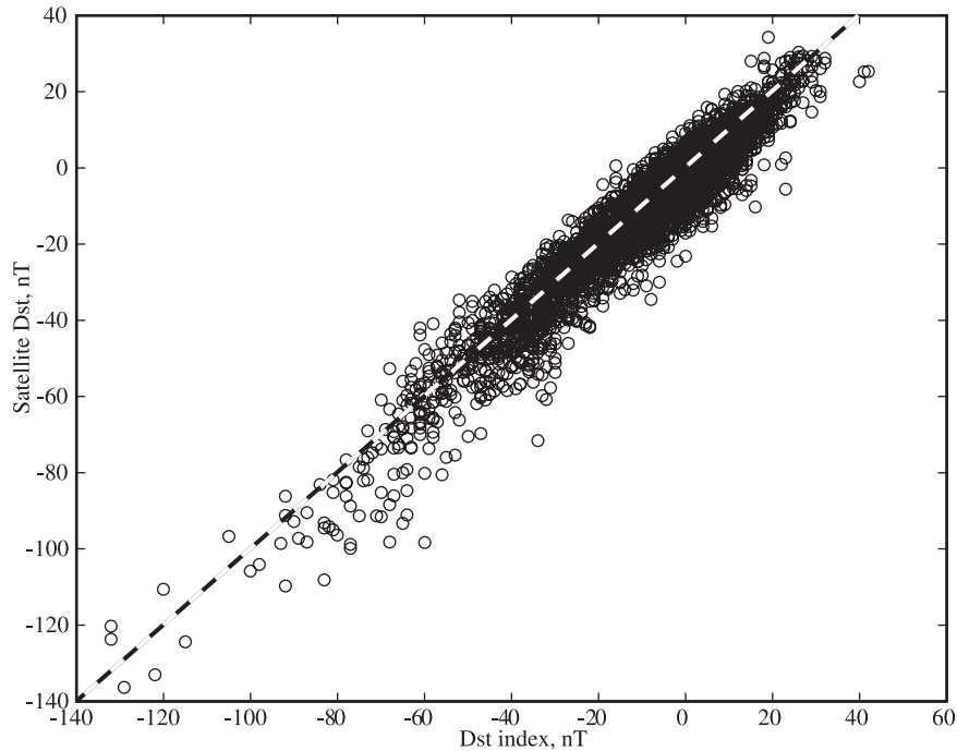
Figure 5. Scatterplot of dawn/dusk average of total field estimated from satellite data ( [e_1^0(t) + i_1^0(t)]/2 ) against the Dst index.
