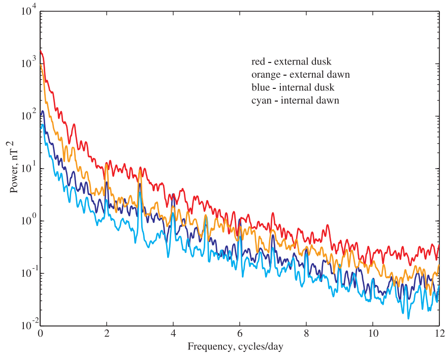
Figure 6. Spectra of the four timeseries shown in Figure 3. It can be seen that the dusk passes have greater power than the dawn passes at all frequencies, and are less contaminated by harmonics of the daily variation.
