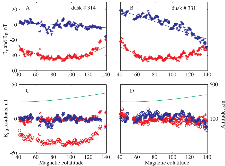
Figure 2. Data, fits, and residuals for two dusk passes. (a, b) Blue represents data (asterisk symbols) and fits (solid lines) to the B_r component and red represents data and fits for the B_\theta component. (c, d) Residuals from these fits are again as shown as colored asterisk symbols. Also shown in the bottom panels are the CMP3 residuals (with the Dst correction turned on) for B_r and B_\theta as blue and red circles symbols respectively. For pass number 331 (right), the CMP3 model does a good job of fitting the storm-time fields, but for pass 314 (left), CMP3 does poorly, as is evident by the large B_\theta residuals. Satellite altitude is shown in green in Figures 2c and 2d.
