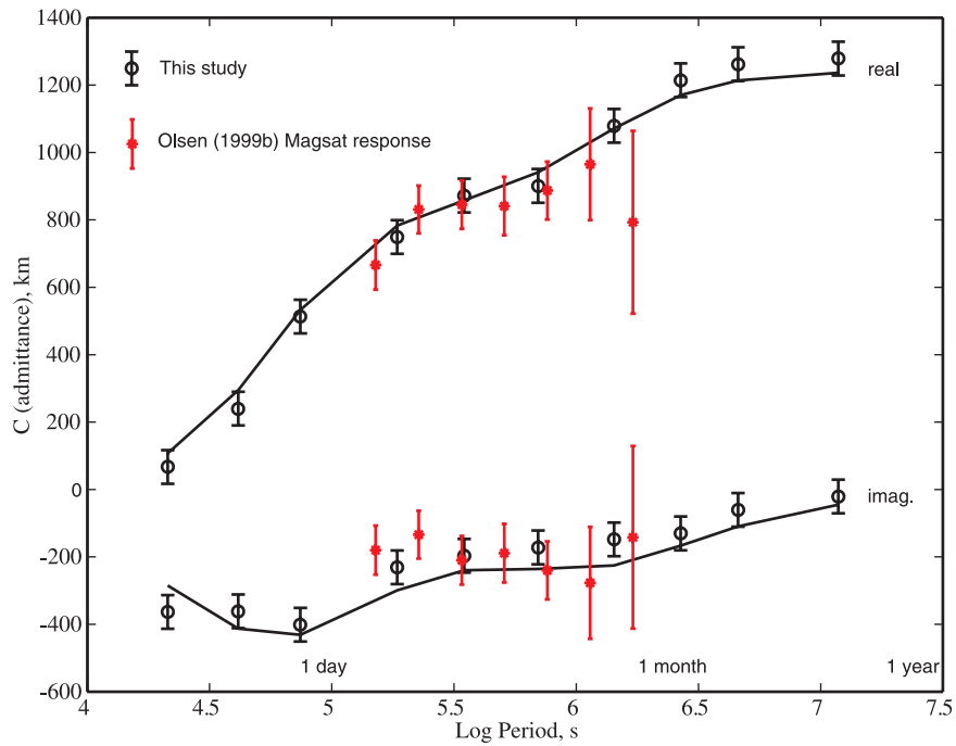
Figure 8. 1-D transfer functions from this study (black), and Olsen's [1999b] study of the same Magsat data set (red). Solid lines show least squares best fitting model responses ( D^+ ) for our data.
