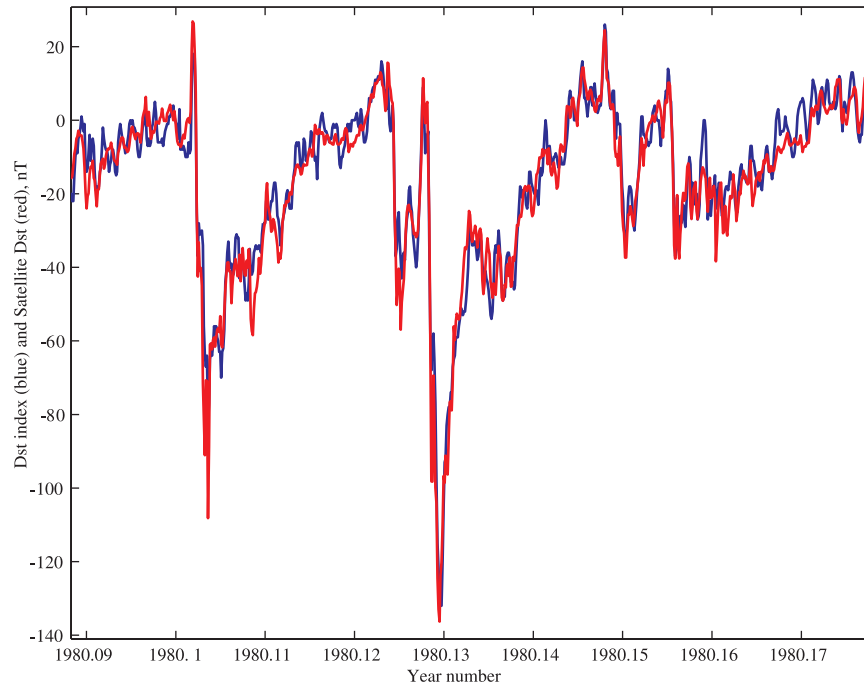
Figure 4. Sum of internal and external field coefficients averaged over dawn and dusk passes (“satellite Dst”, red) compared with the Dst magnetic index (blue).
